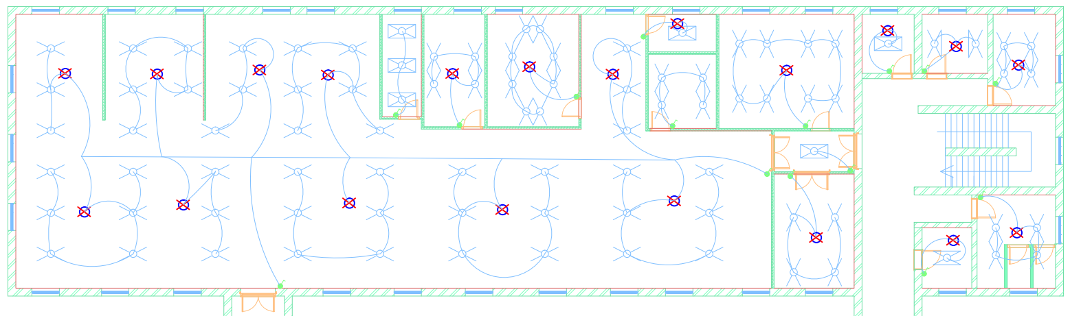
01 LIGHTING LAYOUT 1:100
