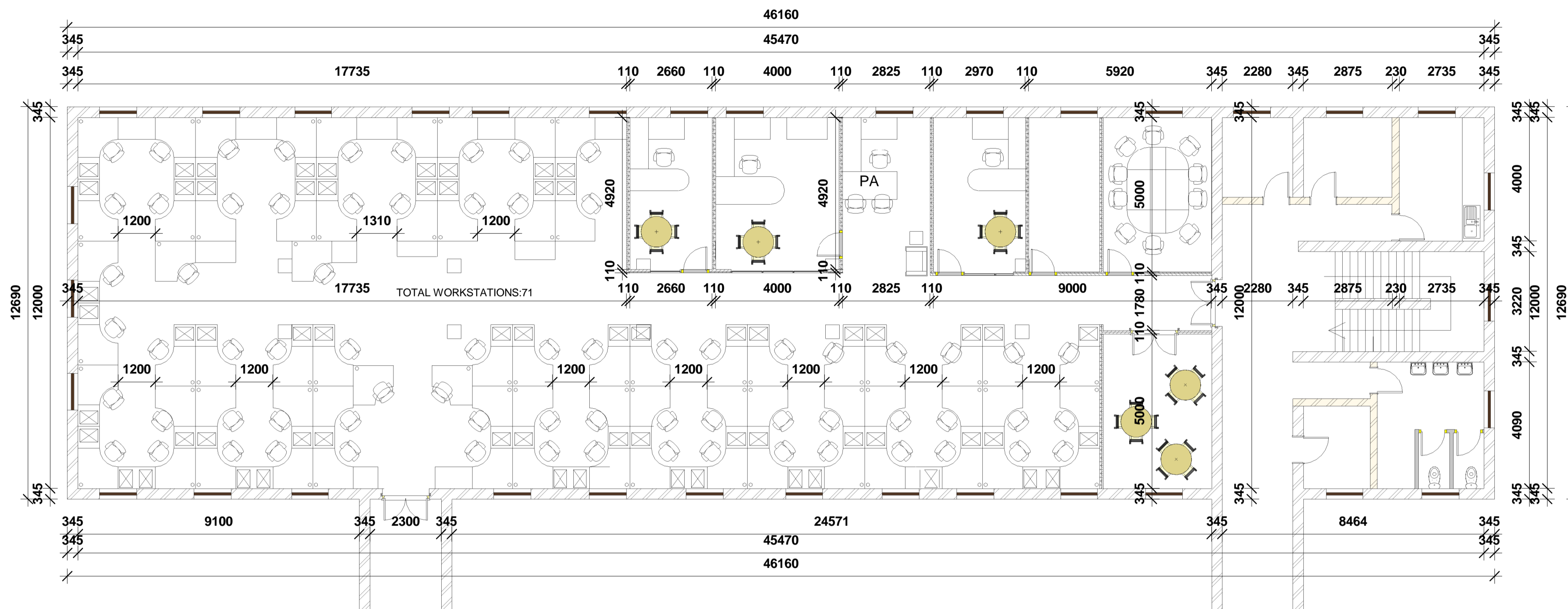
01 FURNITURE LAYOUT 1 : 100
