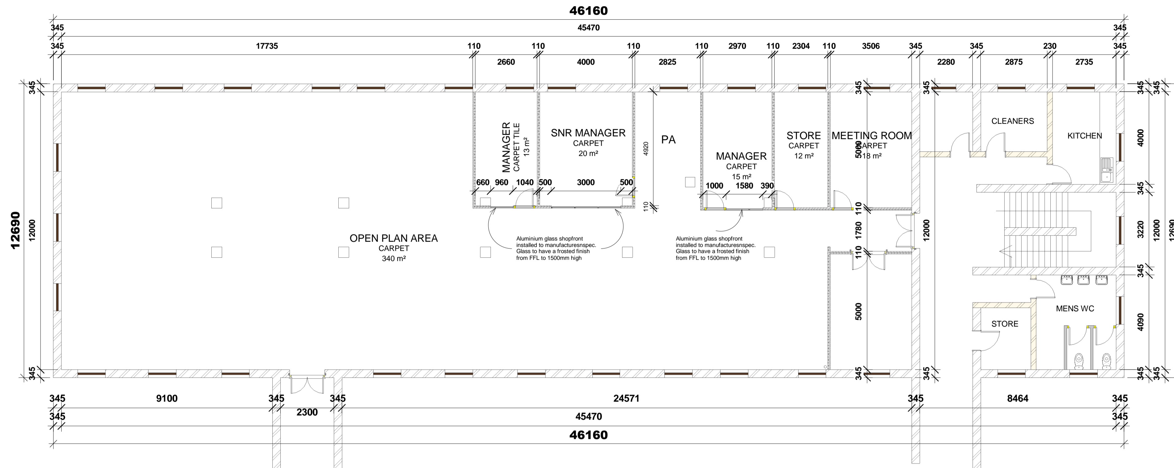
01 GROUND FLOOR PLAN 1 : 100
